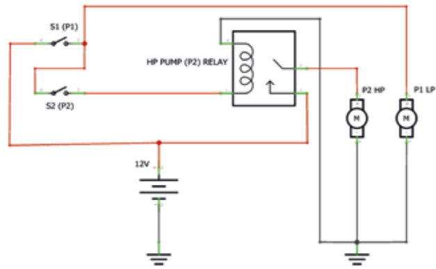
Nautilus WaterBaby 15 - electrical schematic - pump control
